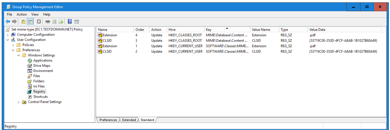
Figure 5. Group Policy Management Editor, Key Locations
