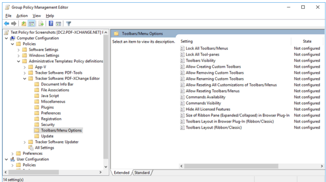
Figure 1. Group Policy Management Editor, Toolbars/Menus Options Category, Available Policies
